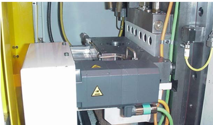
Single Station Shuttle Table Fixture
