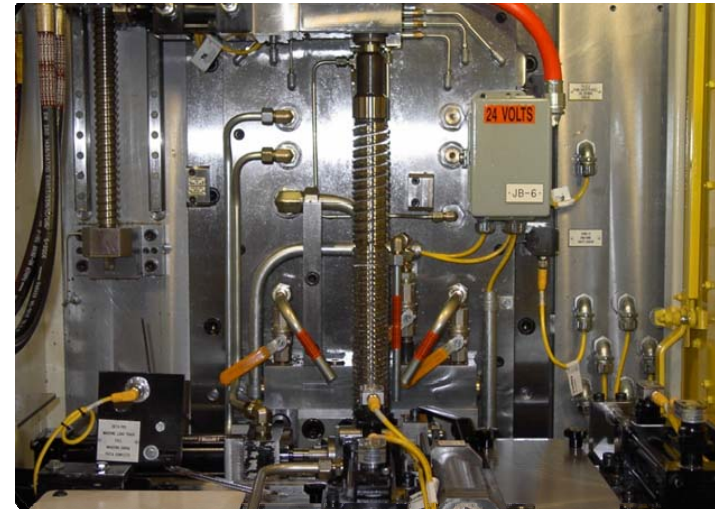
Automatic Load / Unload Fixture w/ Integrated Part Blow-off System
