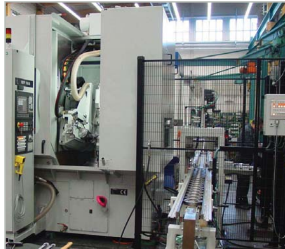
Optional conveyor for in-line automation
