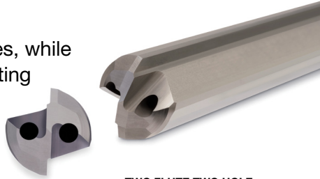
TWO FLUTE TWO HOLE MILLED STYLE GUNDRILL
