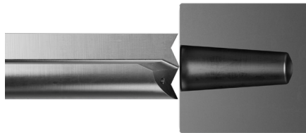
Concave Point Geometry Cutting into a Cored Hole Where the Drill is Larger than the Cored Hole
