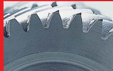
Workpiece after hobbing.
