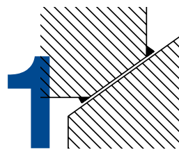
Secondary burr during chamfering
