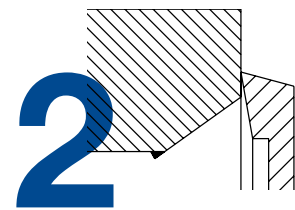
Deburring the secondary burr on gear lateral surfaces
